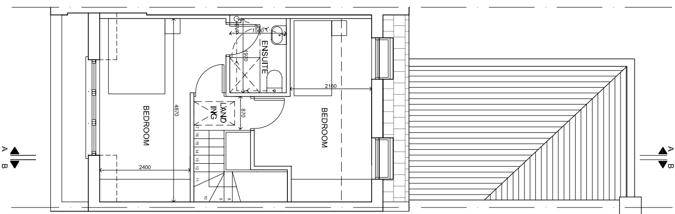
PROPOSED THIRD FLOOR PLAN
